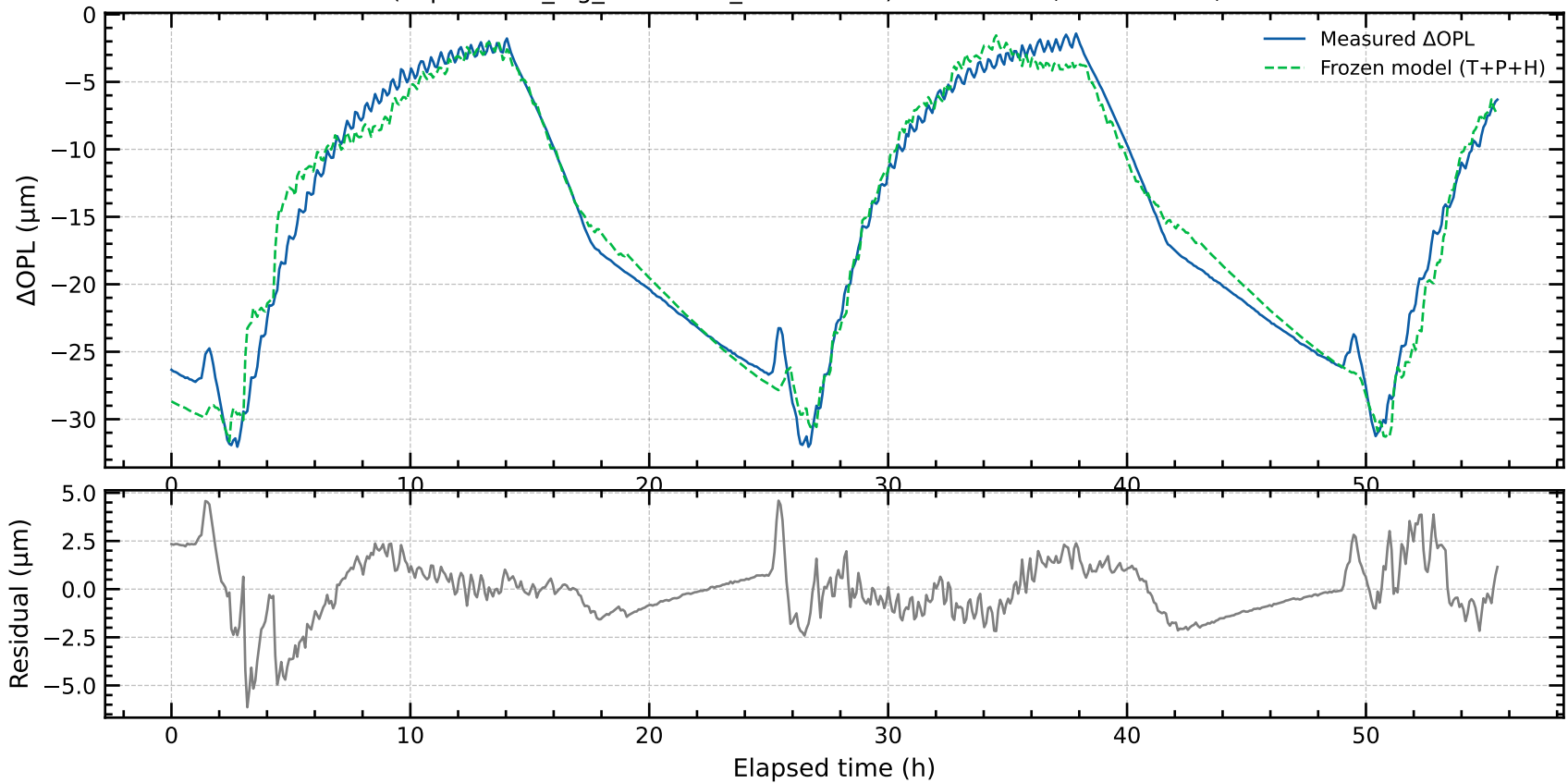
TRAIN (experiment_log_20250425_165701.csv) — R^2=0.972 , RMSE=1.52, MAE=1.16
