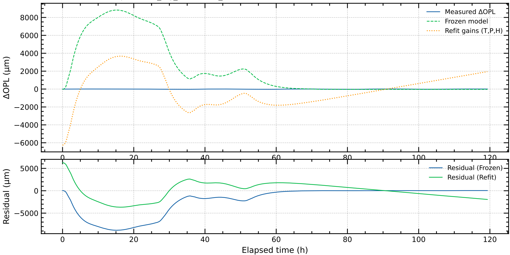
TEST (experiment_log_20250509_202745.csv) — Frozen R^2=-99304.894 , Refit R^2=-26292.093
