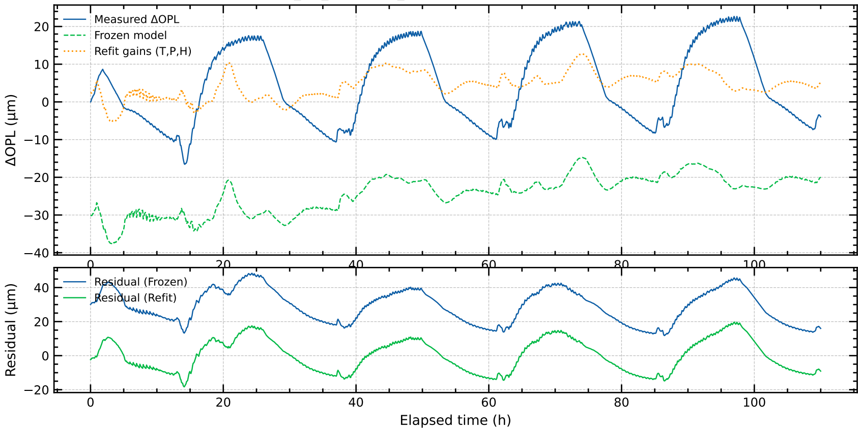
TEST (experiment_log_20250502_170117.csv) — Frozen R^2=-7.531 , Refit R^2=0.162
