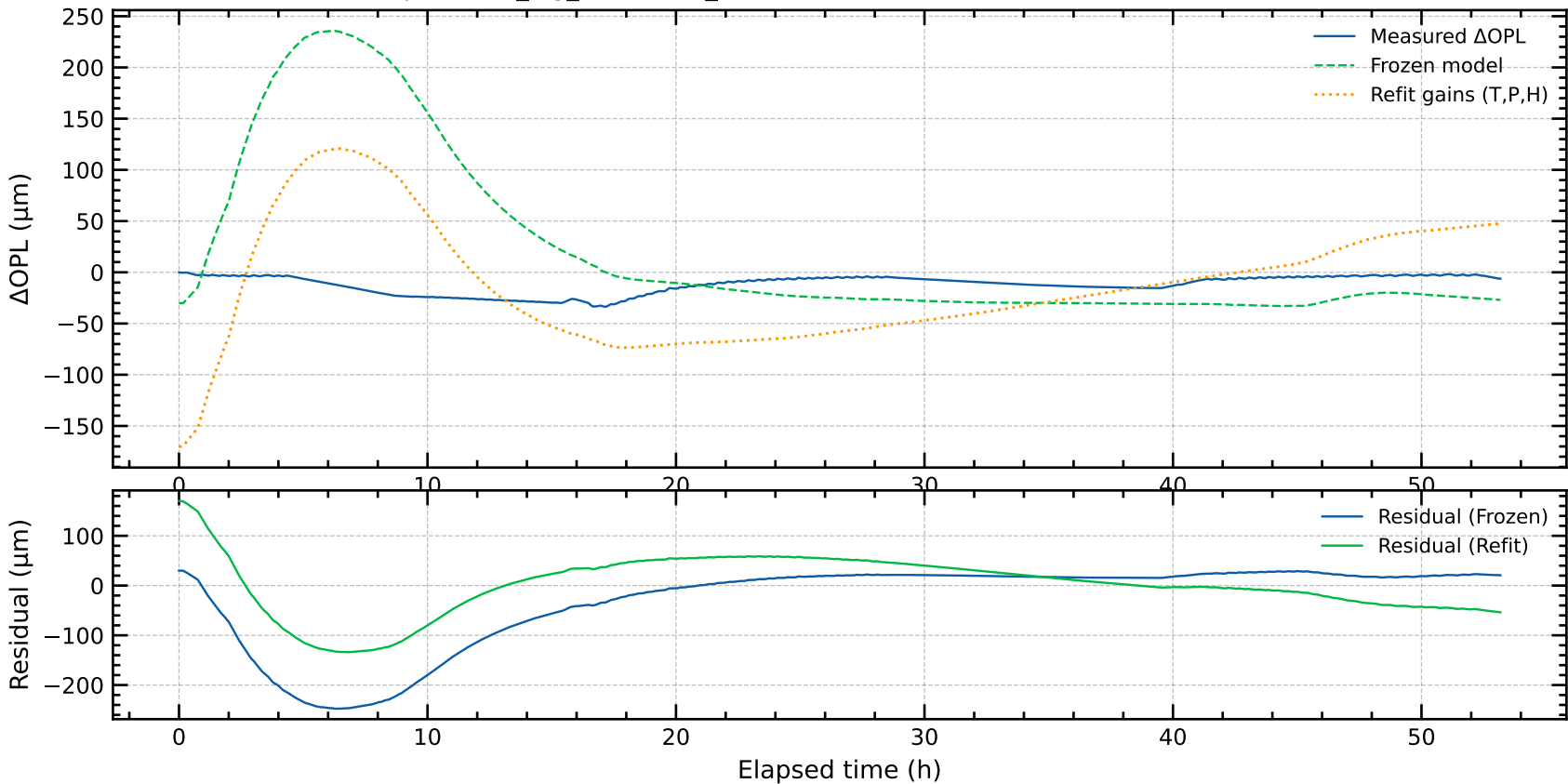
TEST (experiment_log_20250507_143128.csv) — Frozen R^2=-108.537 , Refit R^2=-43.953
